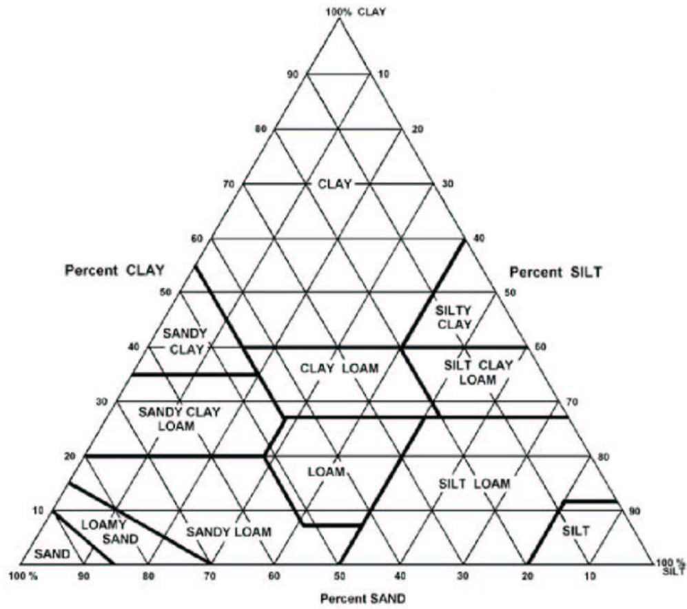
Figure 1: Graph showing the percentages of sand, silt, and clay in the soil texture classes
